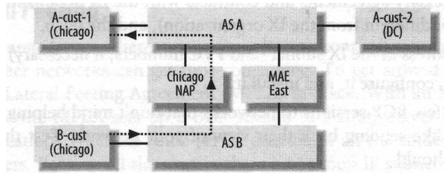
Figure 12-2. Local traffic in early exit routing
